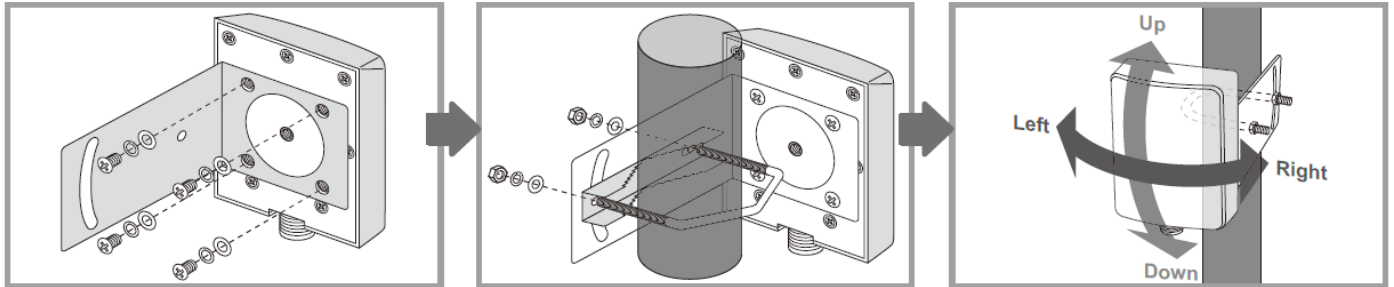
Pole Mount
