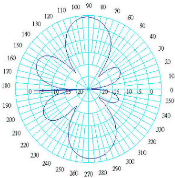
E-PLANE 2.45GHZ=4.397dbi
